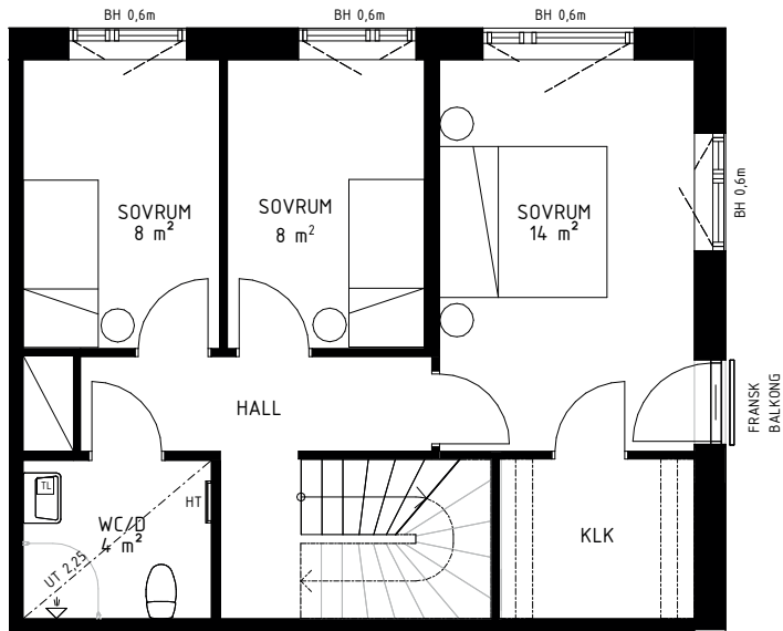
PLAN 2
