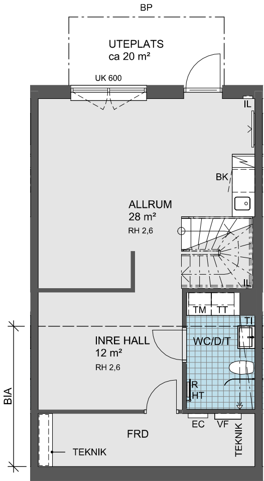
PLAN -1
