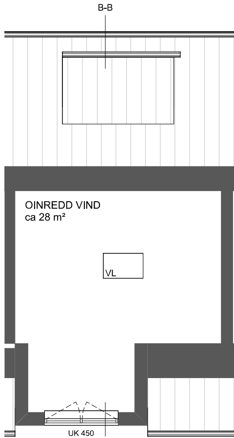
PLAN 3
