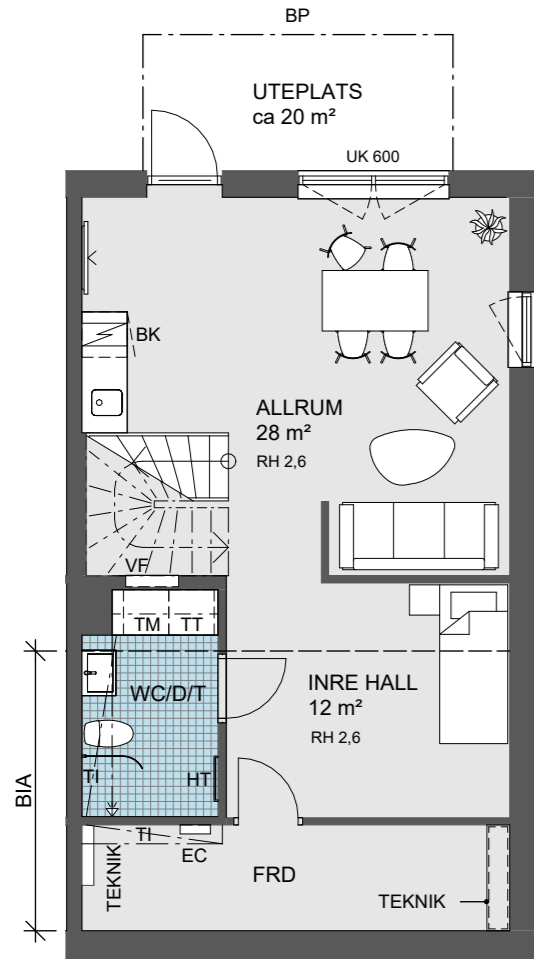
PLAN -1
