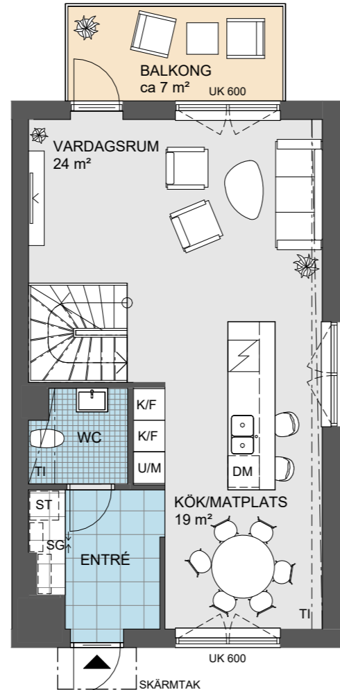
PLAN 1
