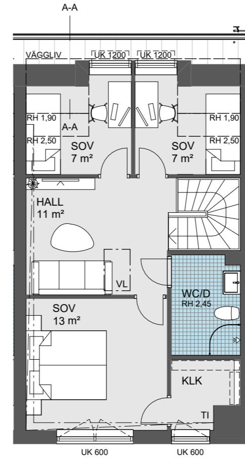
PLAN 2
