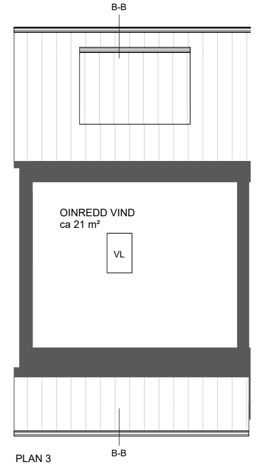
PLAN 3
