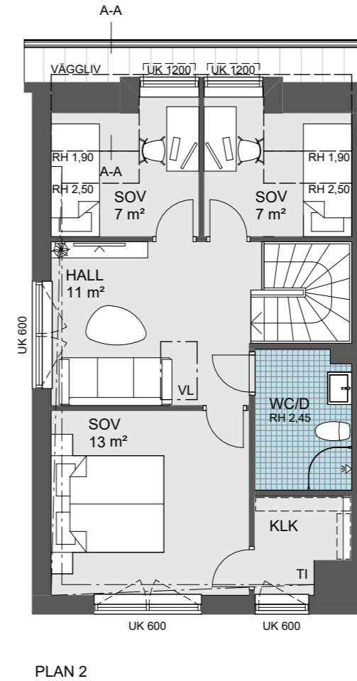
PLAN 2
