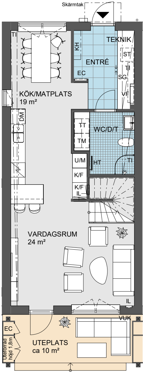
PLAN 1
