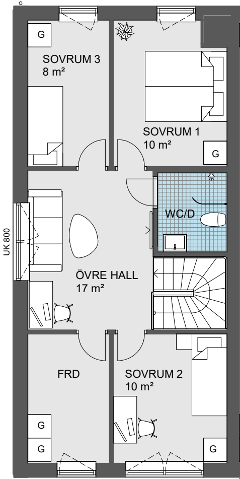
PLAN 2
