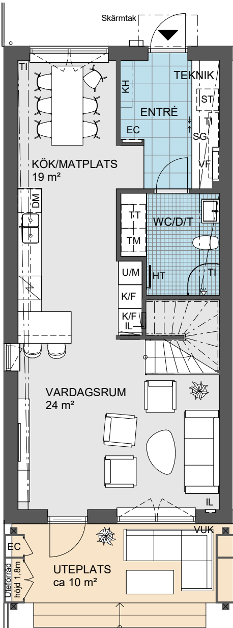
PLAN 1
