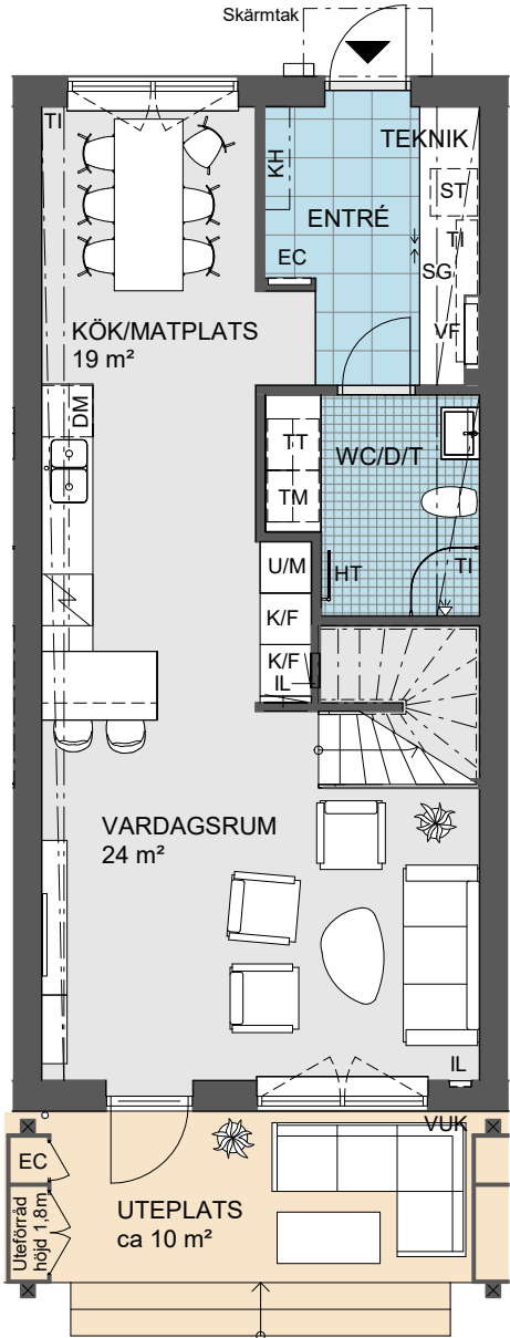
PLAN 1
