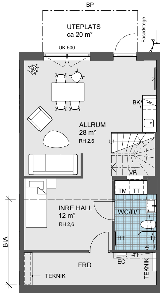
PLAN -1
