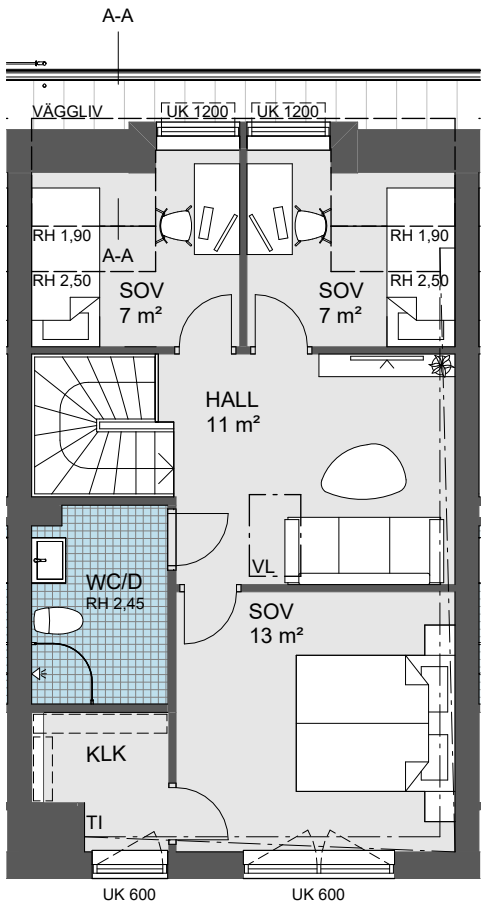
PLAN 2
